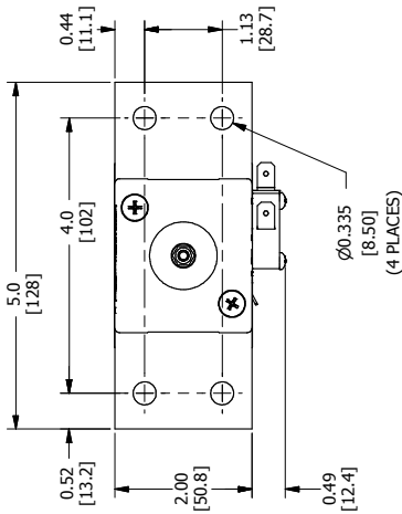
SINGLE POLE SINGLE THROW NORMALLY OPEN
